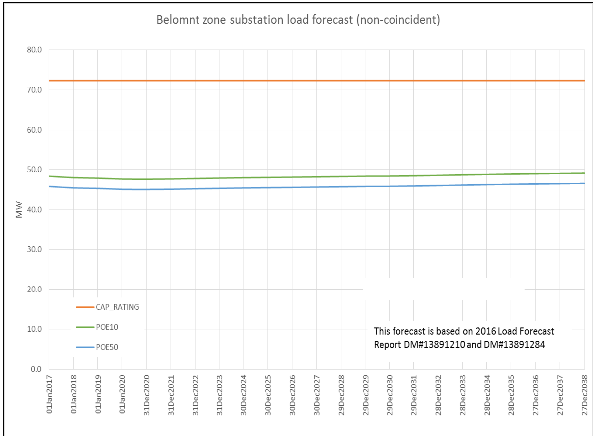
Figure 2 - BEL Zone Substation Forecast
