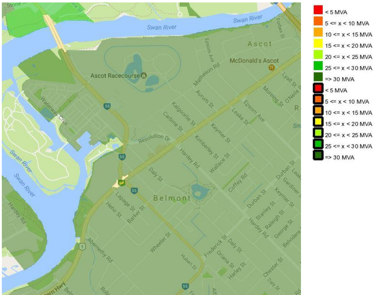
Figure 4-2 Forecast Power Network Capacity 2036 (Source: http://ncmt.westernpower.com.au/index.cfm )
