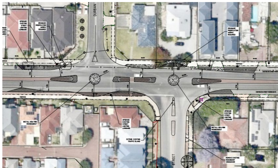
Figure 5: Concept sketch for the proposed roundabouts
