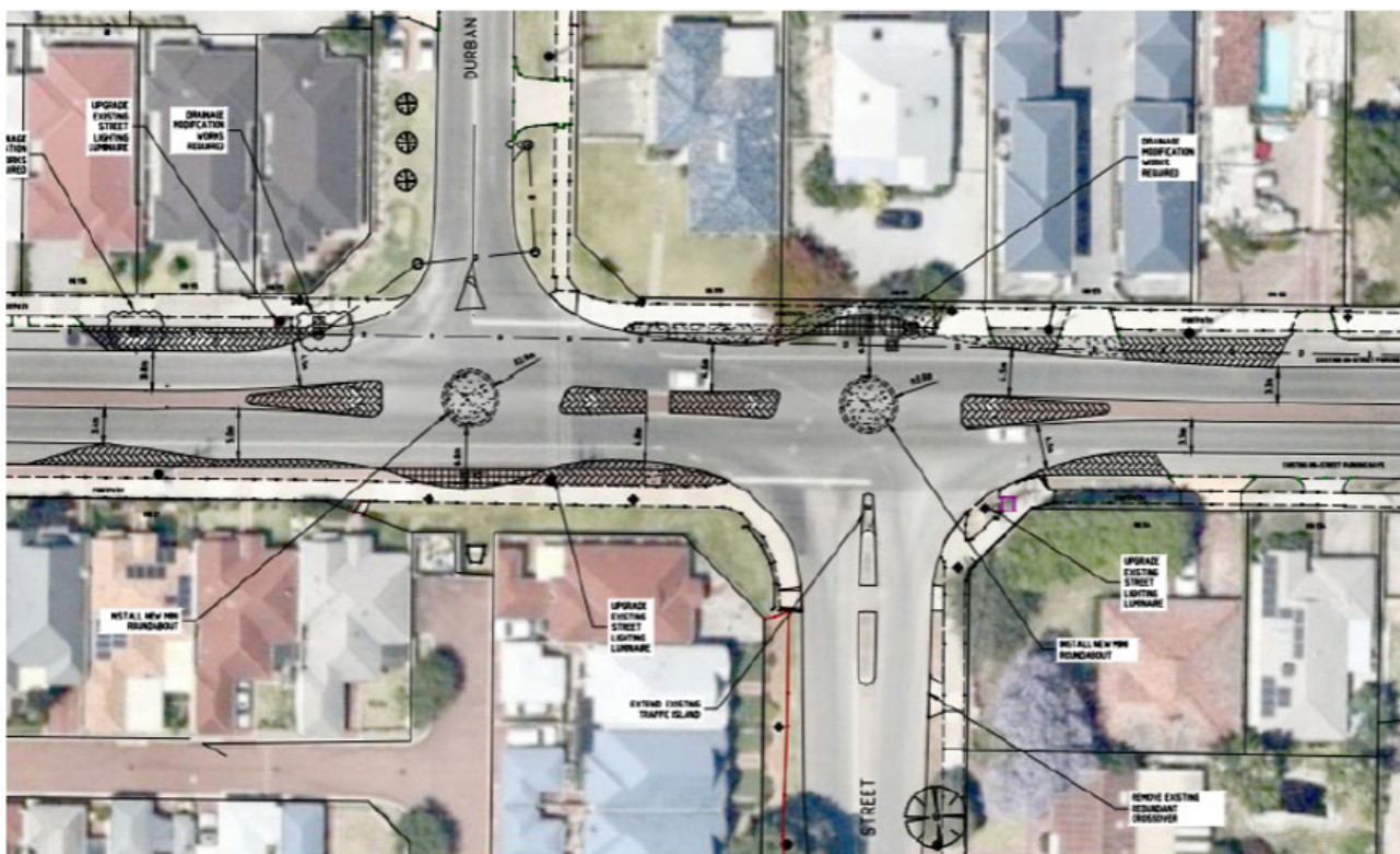
Figure 3: Roundabout upgrade option
